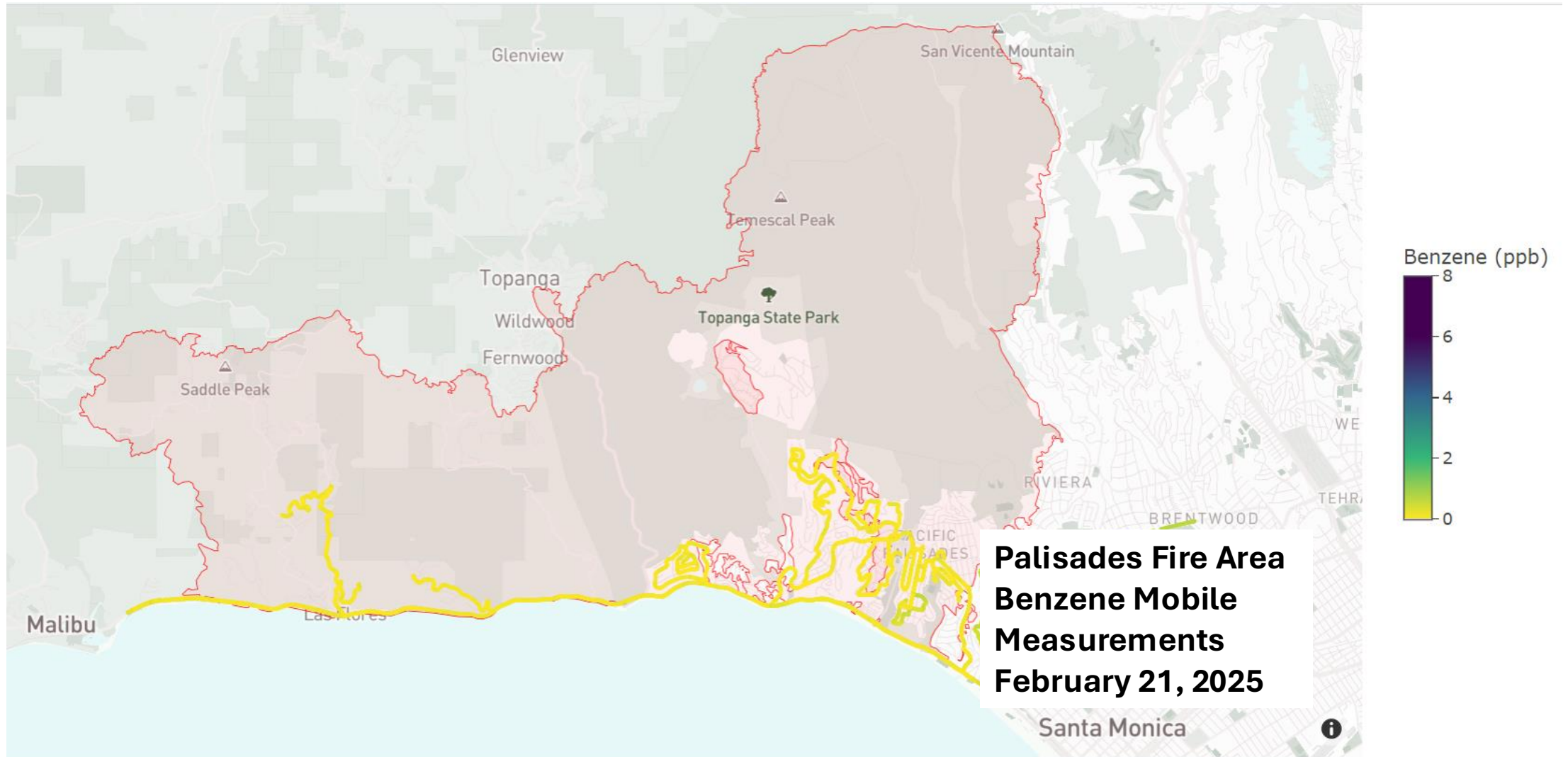
Figure 19. Map shows concentrations of Benzene measured on February 21, 2025.
