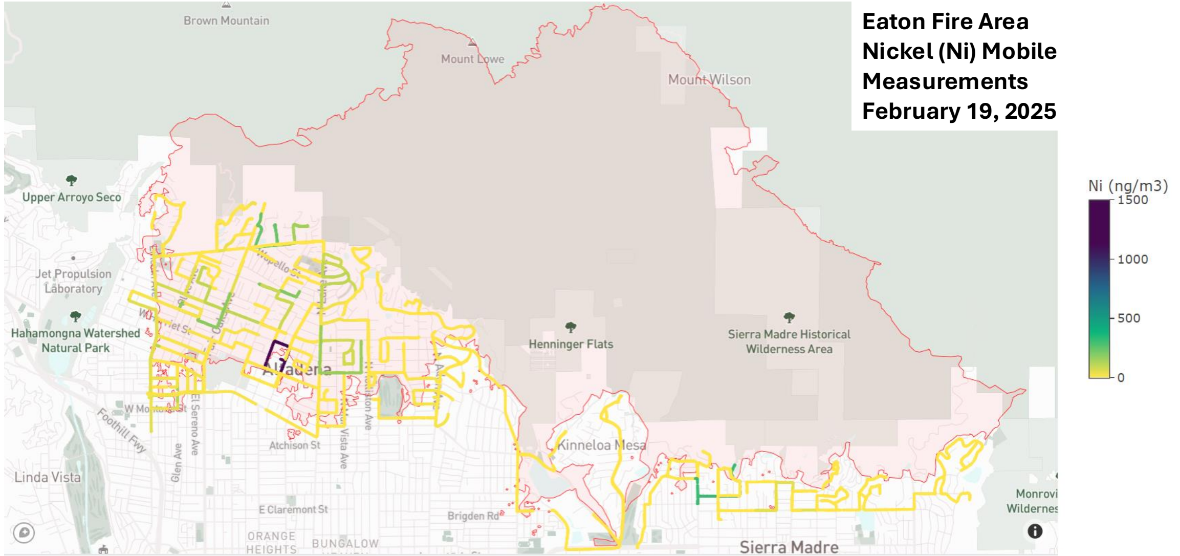
Figure 8. Map shows concentrations of Nickel (Ni) measured on February 19, 2025.
