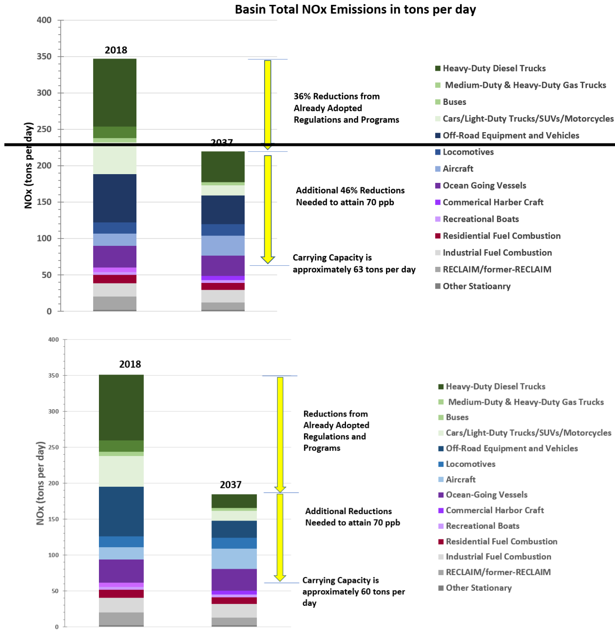
FIGURE 1 BASELINE NO x EMISSIONS INVENTORIES AND ADDITIONAL REDUCTIONS REQUIRED TO ATTAIN THE 2015 8-HOUR OZONE STANDARD
