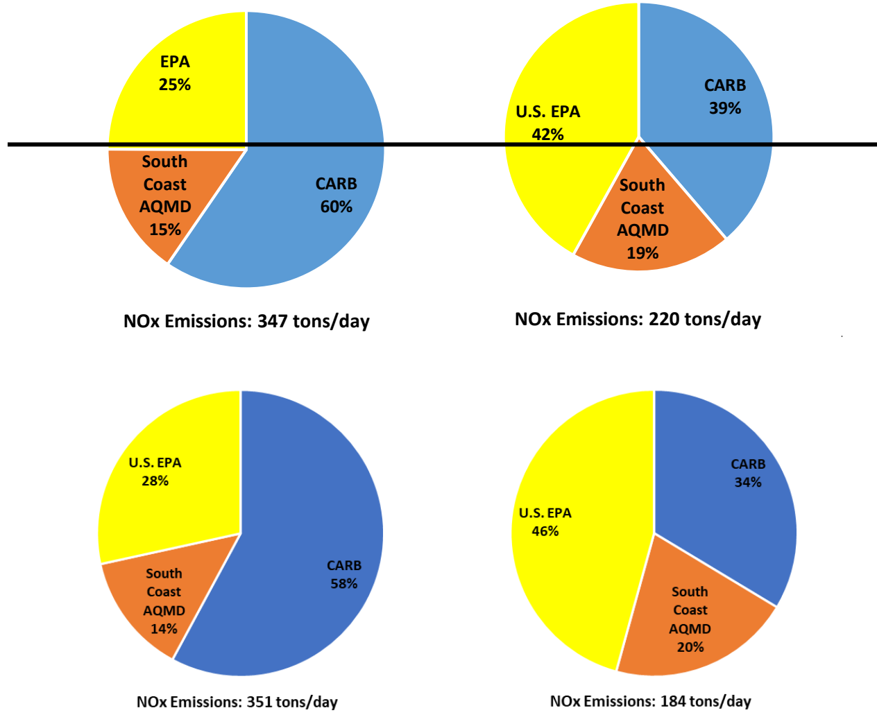
FIGURE 2 2018 (LEFT) AND 2037 (RIGHT) BASELINE EMISSIONS INVENTORY AGENCY RESPONSIBILITY
