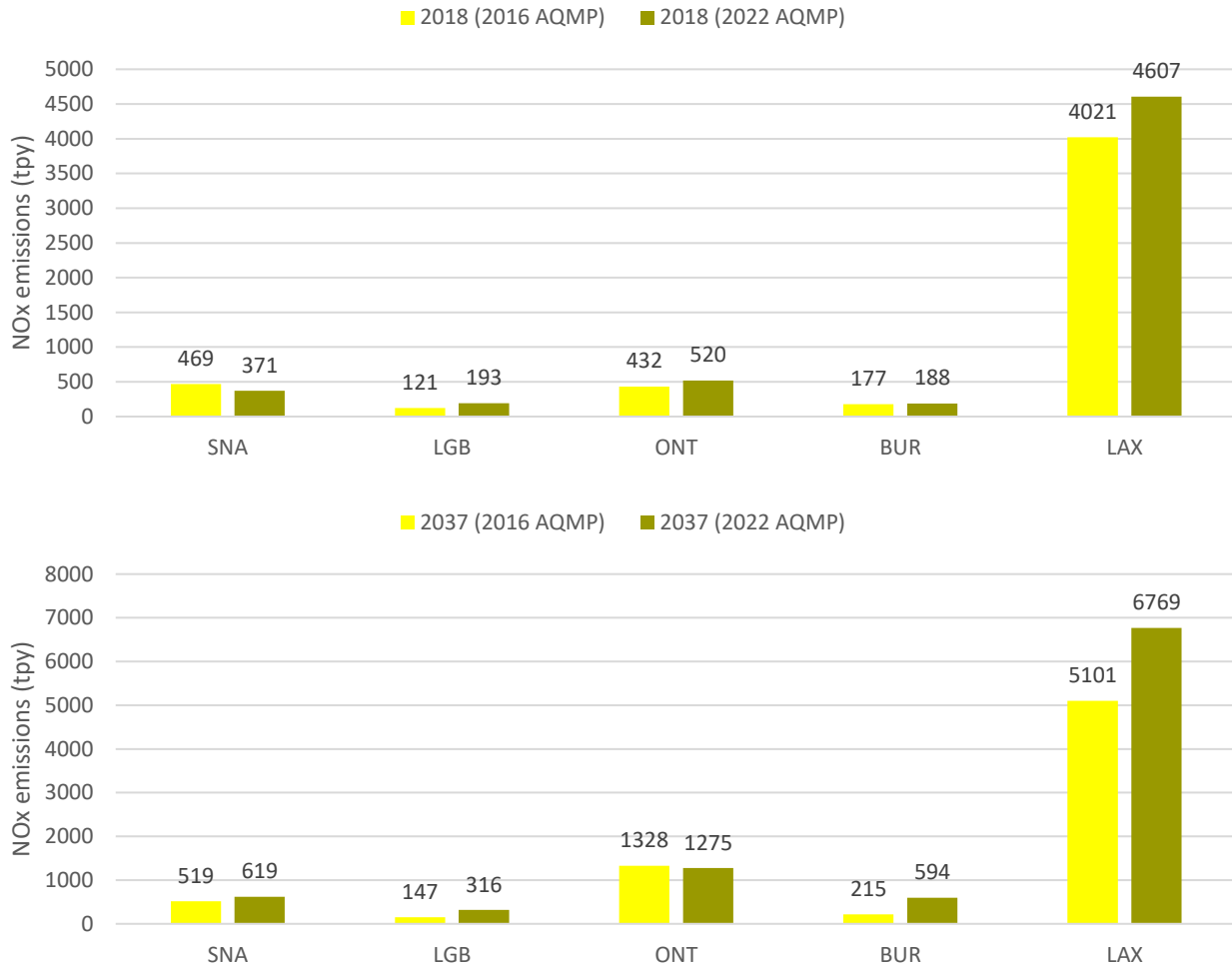
FIGURE III-1-3 AIRCRAFT NOx EMISSIONS IN SCAB COMMERCIAL AIRPORTS FOR THE 2022 AQMP COMPARED TO THE 2016 AQMP INVENTORY FOR 2018 AND 2037
