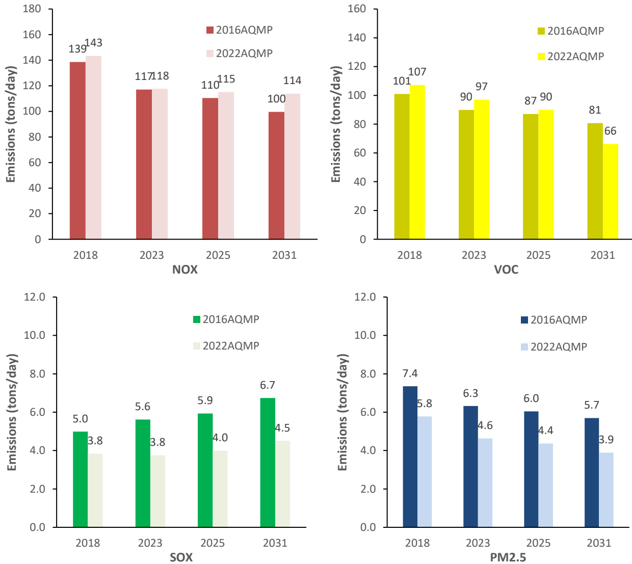
FIGURE III-1-4 COMPARISON OF OFF-ROAD EMISSIONS - 2016 AQMP AND 2022 AQMP (SUMMER PLANNING INVENTORY)
