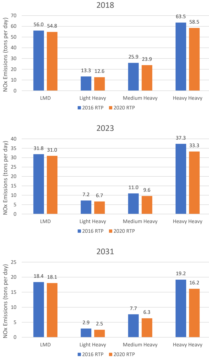
FIGURE III-1-2B COMPARISON OF NOX SUMMER PLANNING EMISSIONS ESTIMATED WITH TRAVEL ACTIVITY DATA FROM 2016 RTP VS. 2020 RTP (USING EMFAC 2017 WITH OFF-MODEL ADJUSTMENTS)
