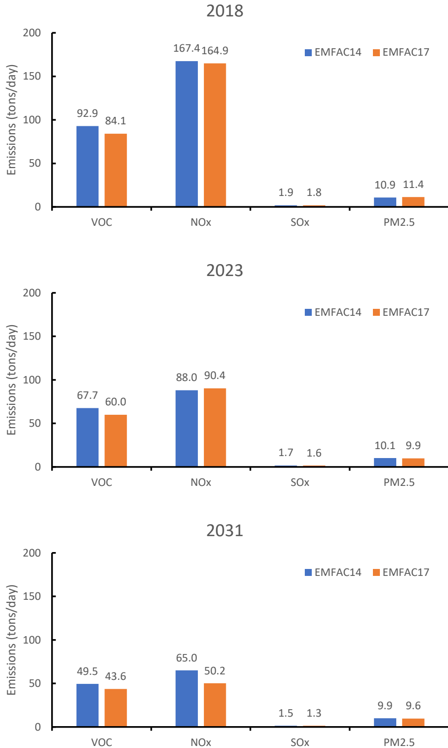
FIGURE III-1-2C COMPARISON OF ON-ROAD SUMMER PLANNING EMISSIONS ESTIMATED BY EMFAC 2014 VS. EMFAC 2017 WITH OFF-MODEL ADJUSTMENTS (USING TRAVEL ACTIVITY DATA FROM 2016 RTP)
