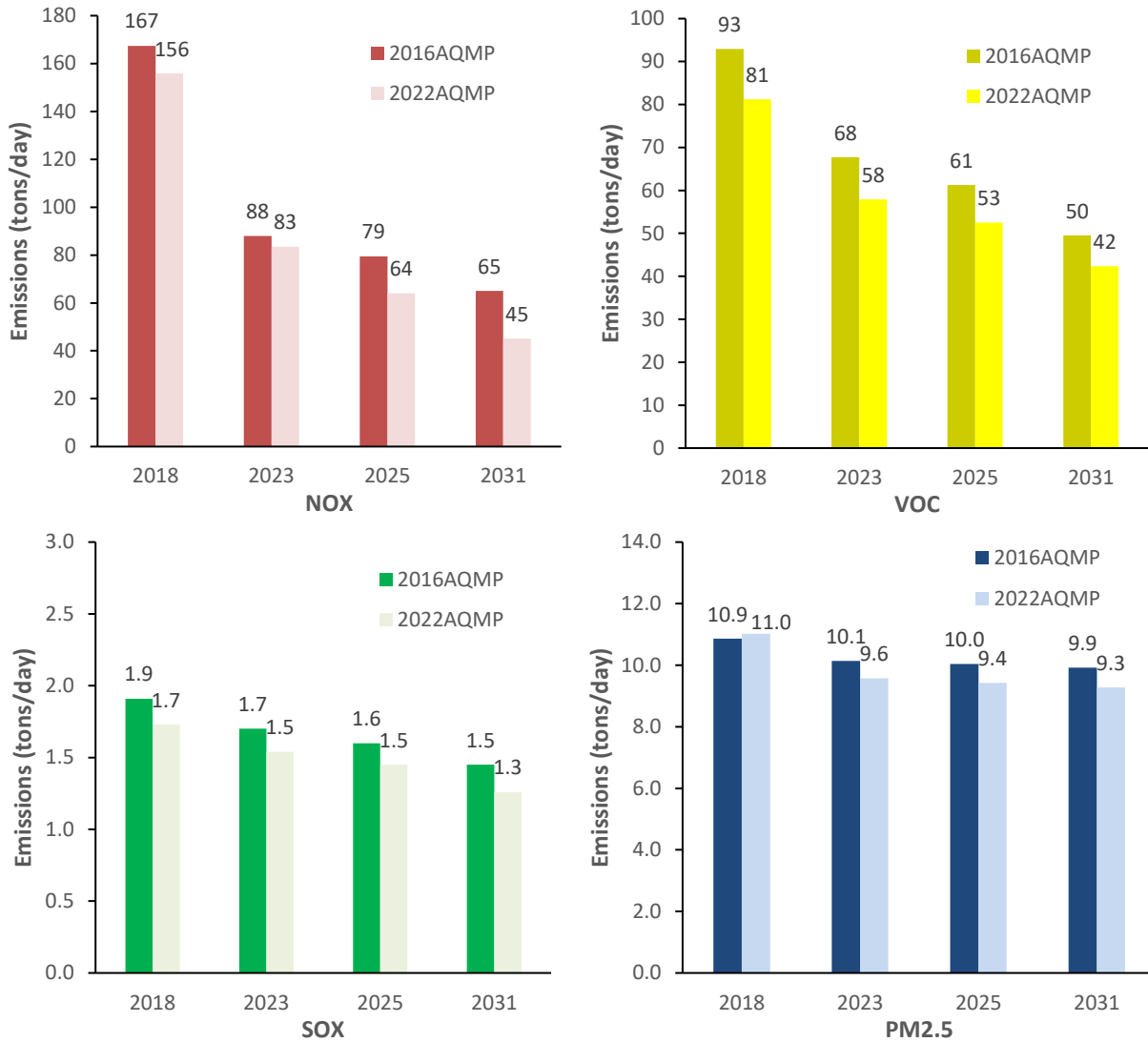
FIGURE III-1-2A COMPARISON OF ON-ROAD EMISSIONS OF BASE AND FUTURE MILESTONE YEARS IN 2016 AQMP AND 2022 AQMP (SUMMER PLANNING INVENTORY)
