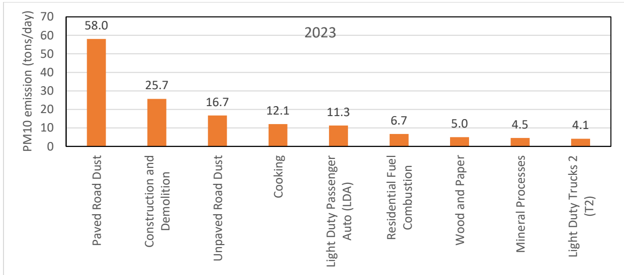
Figure 3-3-A. Top 9 PM10 sources in 2023
