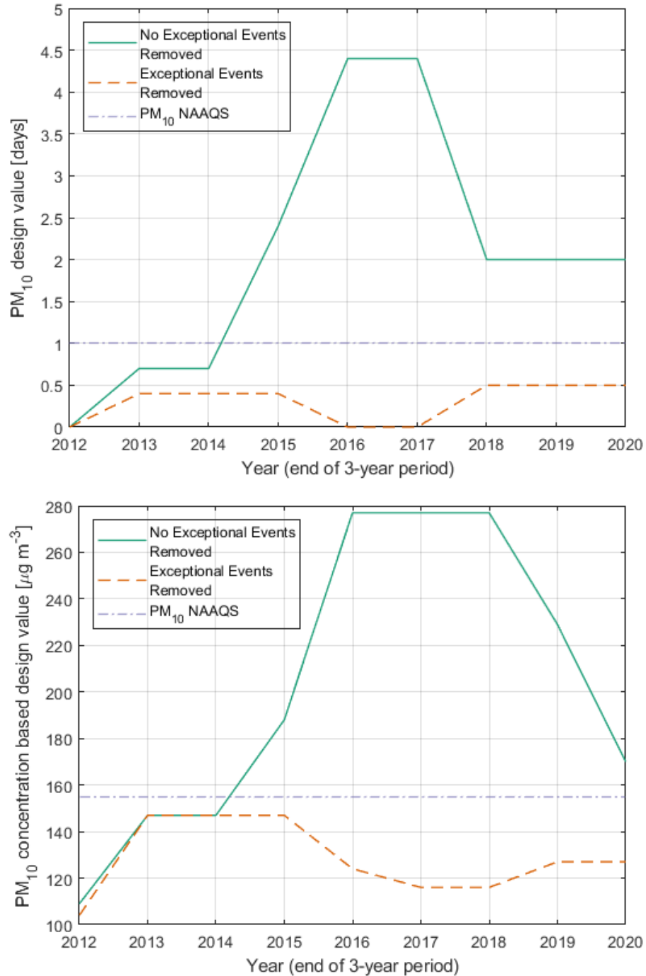
Figure 2-4: Trend of PM 10 design values (top) and concentration-based design value (bottom). The value shown is the maximum of all PM 10 monitors in the South Coast Air Basin.
