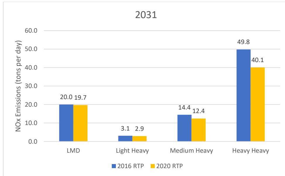
Figure 3-1-C: 2031 NOx emissions estimated with travel activity data from 2016 RTP vs 2020 RTP
