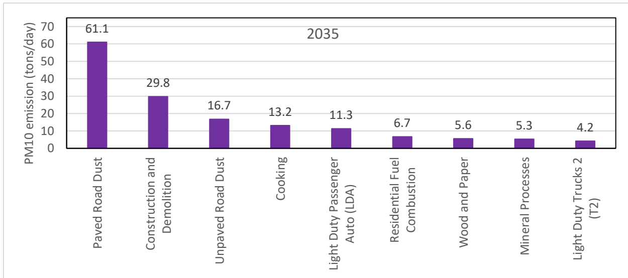
Figure 3-3-C. Top 9 PM10 sources in 2035
