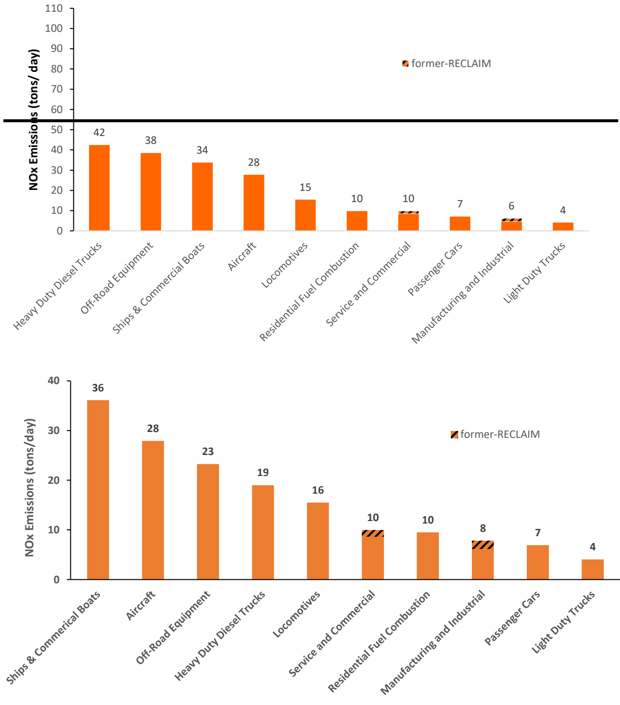
FIGURE 3-10 TOP TEN EMITTER CATEGORIES FOR NO x IN 2037 (SUMMER PLANNING, FORMER-RECLAIM PORTION OF EACH SOURCE CATEGORY IS SHOWN WITH HATCHED AREAS)
